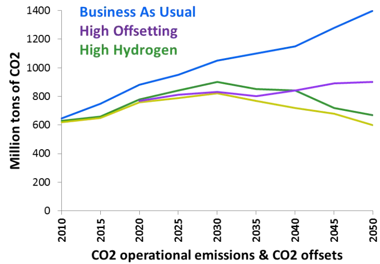
LR Carbon Pathways – Shipping GHG Emissions Scenarios
